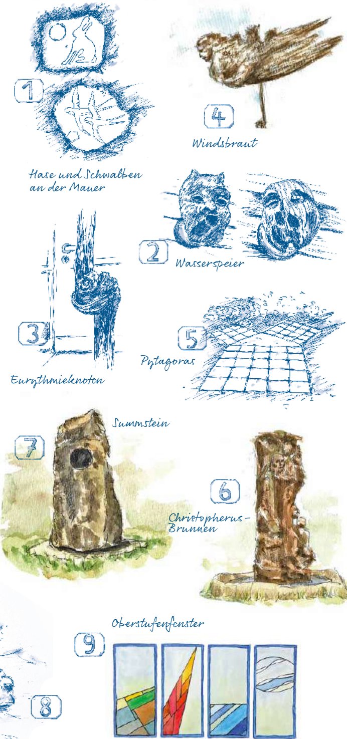
Pythagoras
